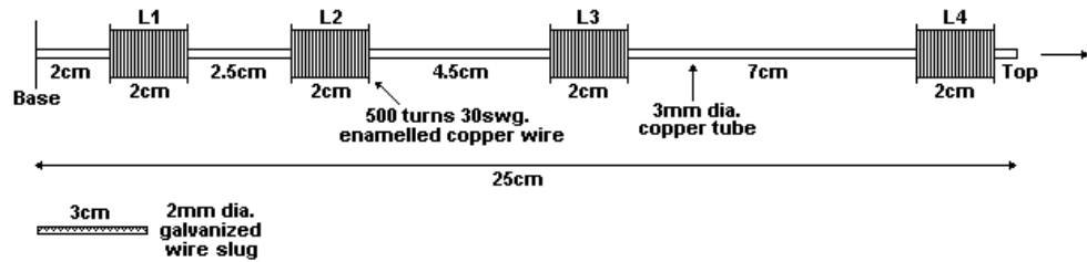
Figure 2. (Mount vertically).
